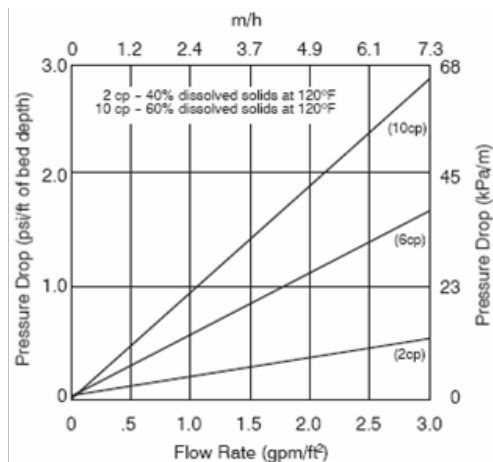
Figure 2: Pressure Drop
