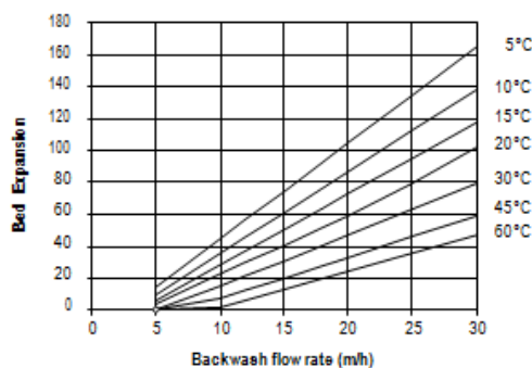
Figure 1: Backwash Expansion
