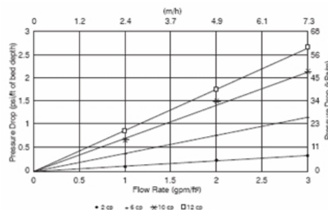
Figure 2: Pressure Drop
