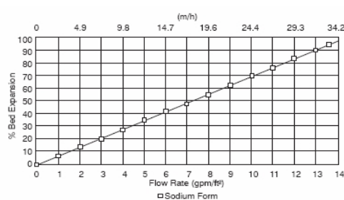
Figure 1: Backwash Expansion
