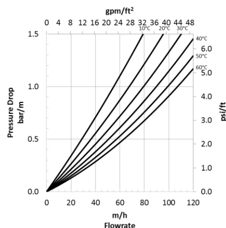
Figure 2: Pressure Drop
