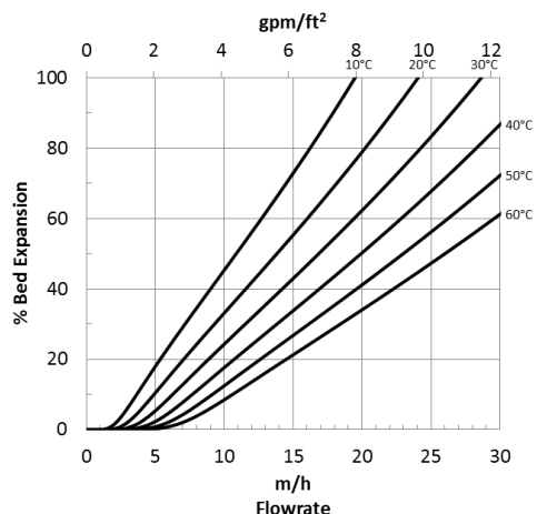
Figure 1: Backwash Expansion
