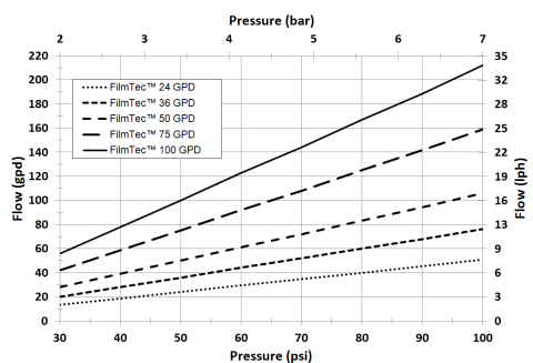
Figure 1: Impact of Pressure on Target Permeate Flow (constant temperature, recovery)
