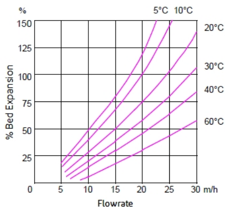
Figure 1: Backwash Expansion
