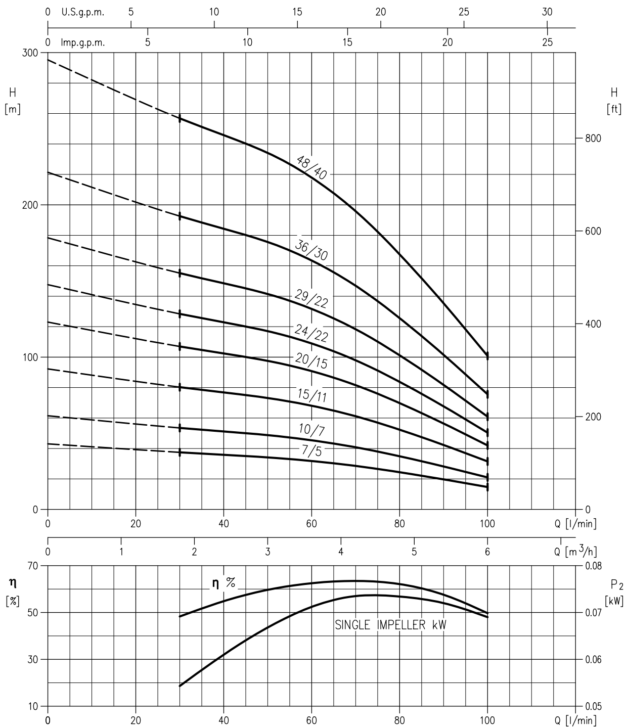
4BHS4 - MEI > 0.70- Impeller diameter = 72 mm
