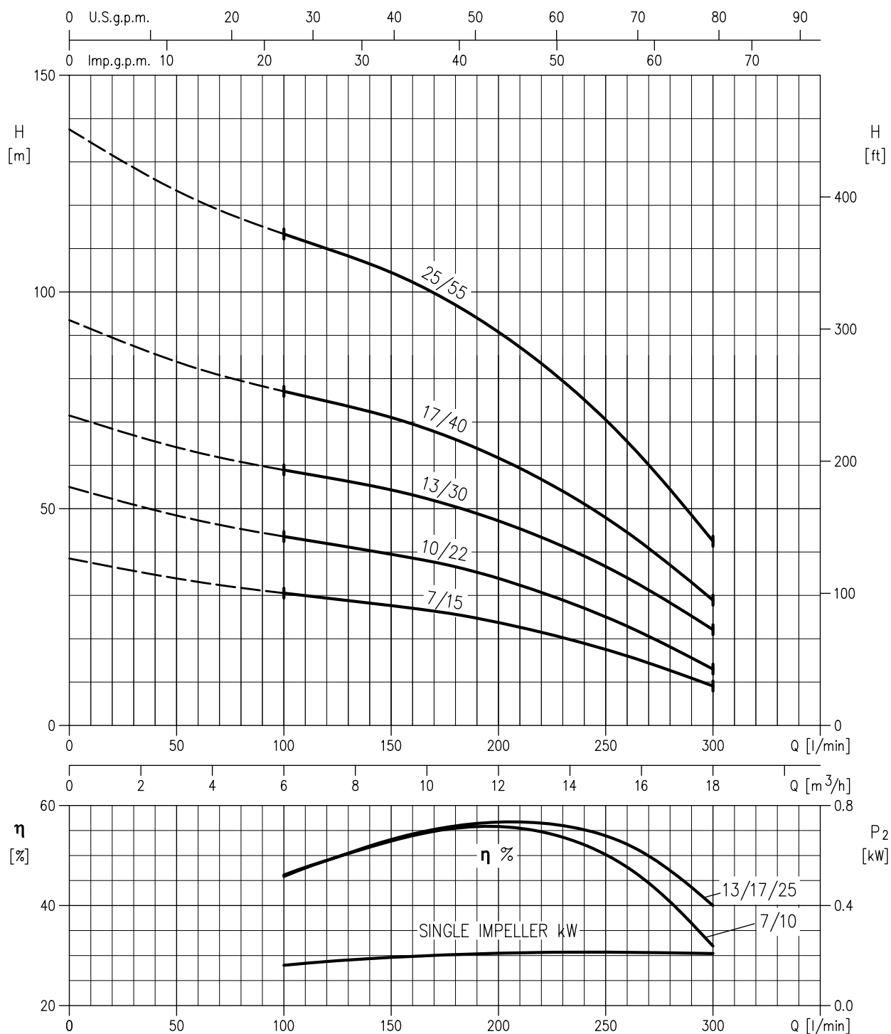
4BHS15 - Impeller diameter = 72 mm
