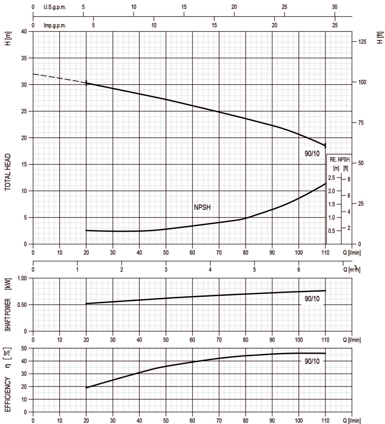
CD 90/10 (0.75 kW) MEI &gt; 0.50 - Impeller diameter = 157 mm
