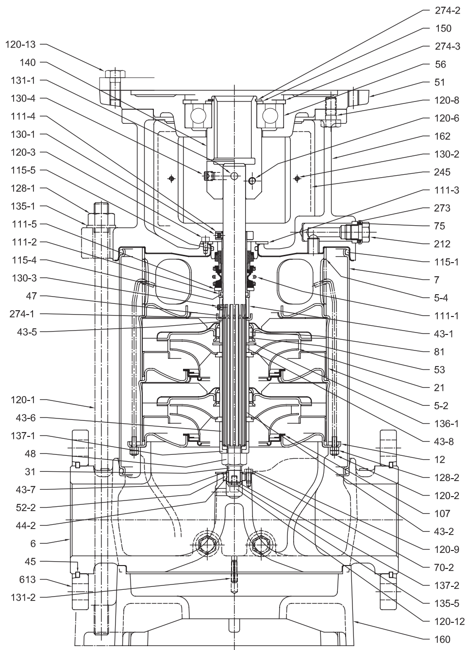
Pump with single ball bearing
