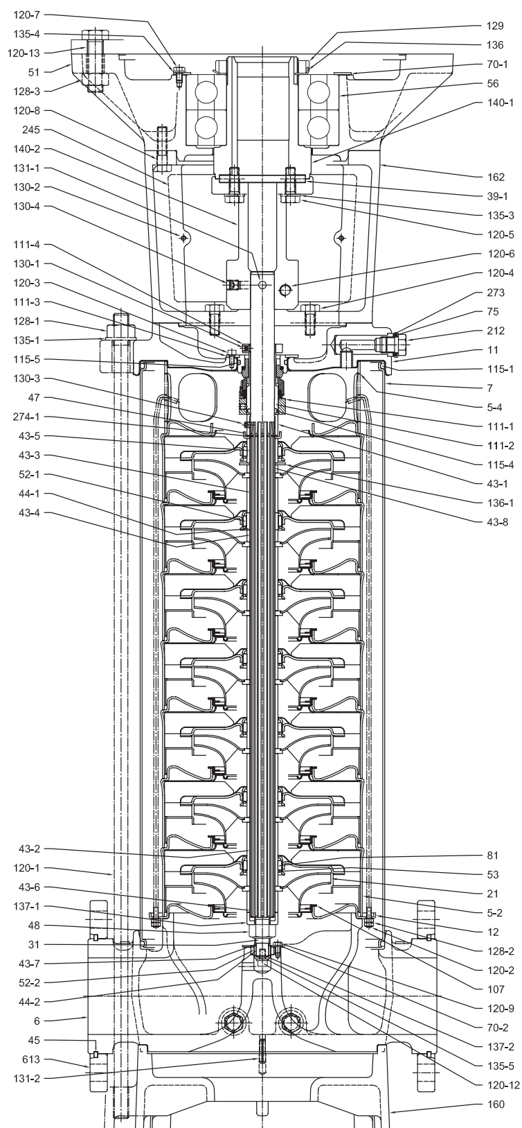
Pump with double ball bearing
