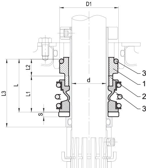
up to 25 bar Cartridge Unbalanced type
