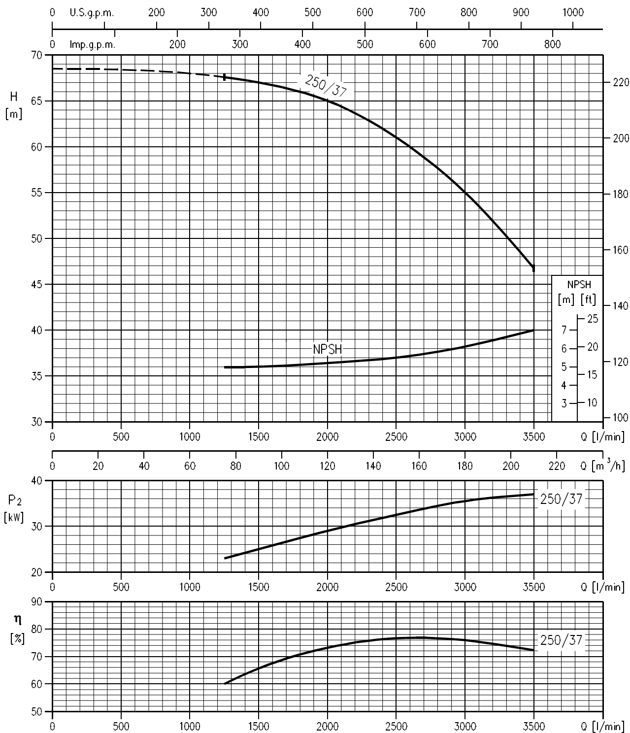
LPC 100-250/37 (37 kW) MEI &gt; 0.40 Impeller diameter = 226 mm
