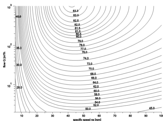
MEI=0.7 for ESCCi 2900 rpm
