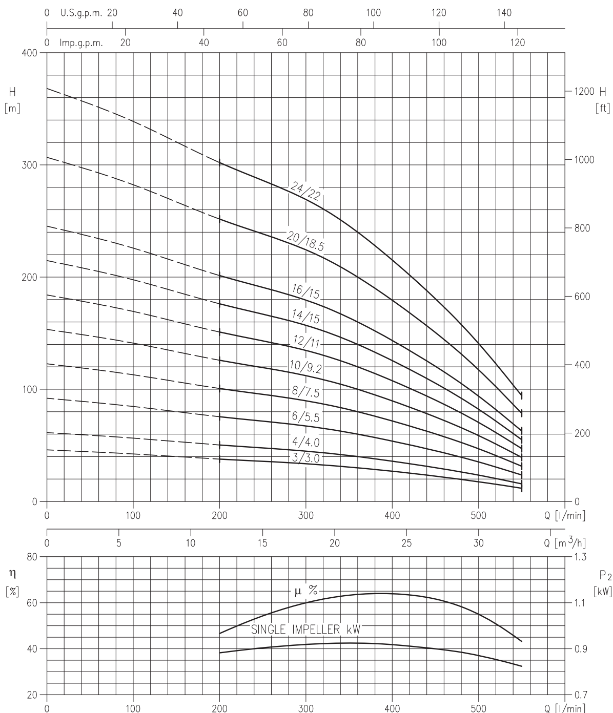
SF6 S25 - Impeller diameter = 111.5 mm
