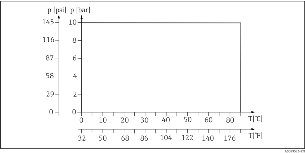
7 Pressure-temperature ratings
