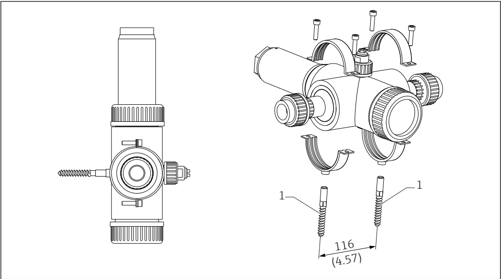
10 Wall mounting kit, dimensions in mm (in) 1 Hanger bolt STST 10 × 60 mm
