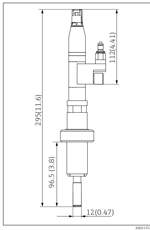
14 Sensor with process connection socket DN30, dimensions: mm (in)
