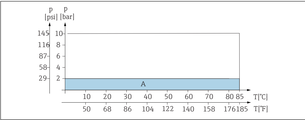
6 Pressure/temperature ratings
