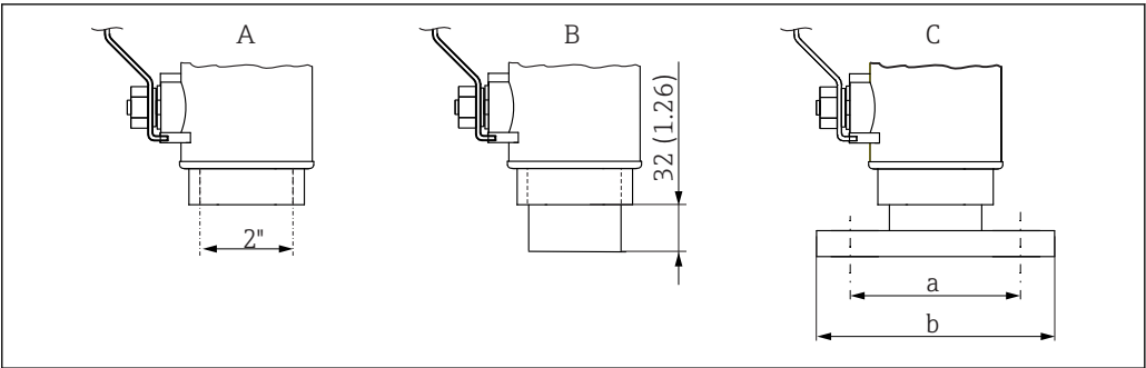
11 Dimensions of process connections in mm (in)
