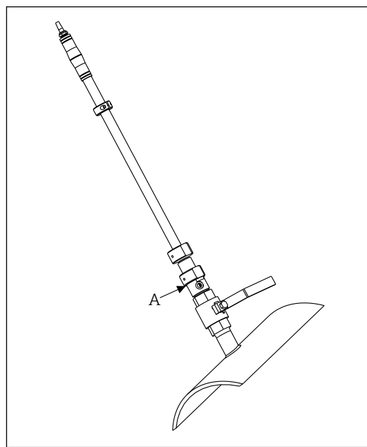
4 Service position (ball valve is closed): assembly is extended for electrode replacement, calibration, rinsing
