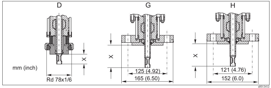
Process connections
