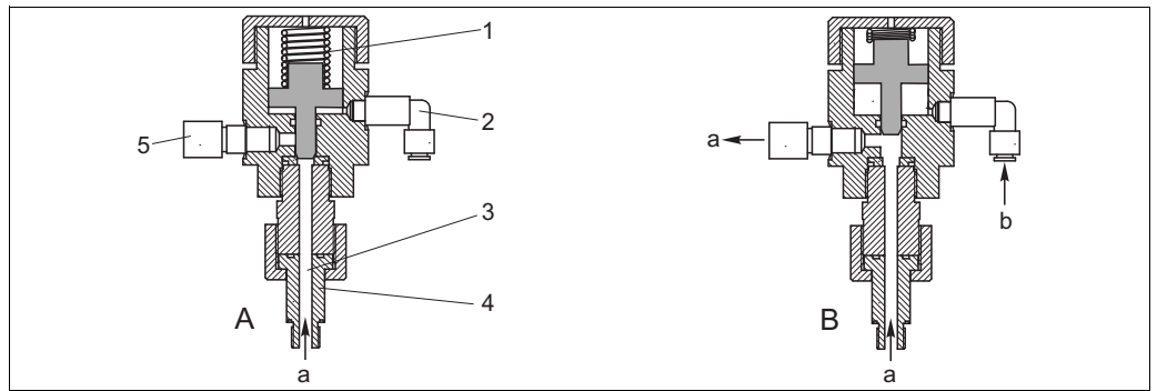
Fig. 7: Functional diagram of the pneumatic valve on the outlet side of the rinse chamber
