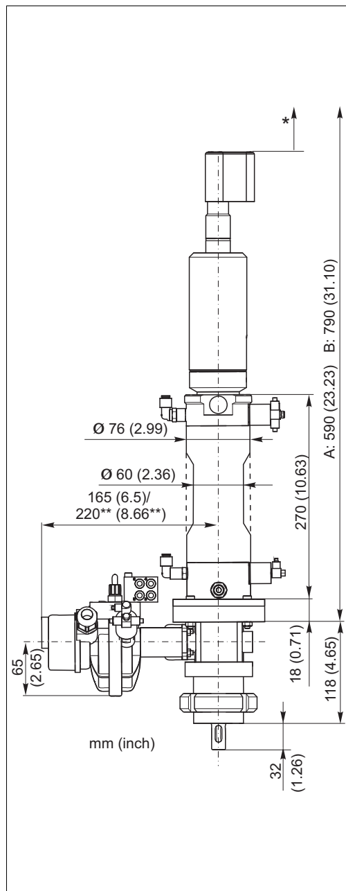
Fig. 4: Assembly version: pneumatic, short, for KCI sensors, thread adapter nut
