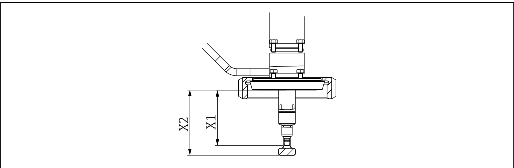
24 Immersion depth in mm (in) for process connection MB thread
