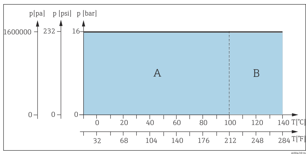
10 Pressure-temperature ratings for pneumatic drive
