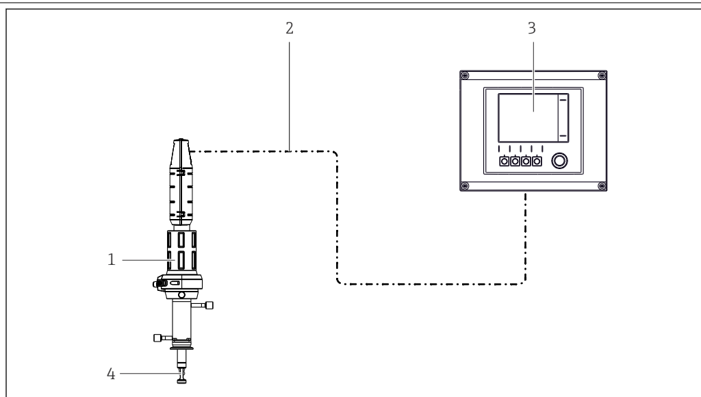
6 Measuring system (example)
