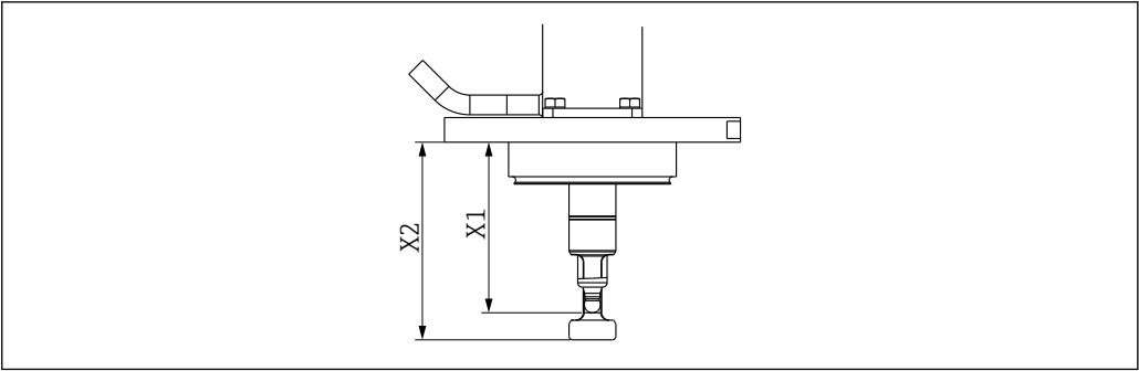
30 Immersion depth in mm (in) for process connection EA thread
