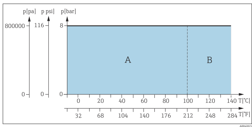
11 Pressure-temperature ratings for manual drive
