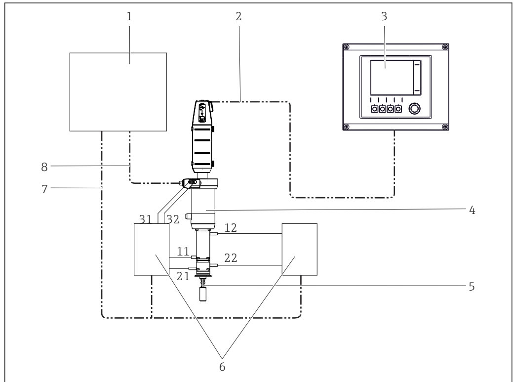
7 Measuring system with pneumatic drive and double chamber (example)
