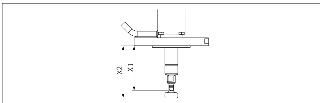
29 Immersion depth in mm (in) for process connection EB thread
