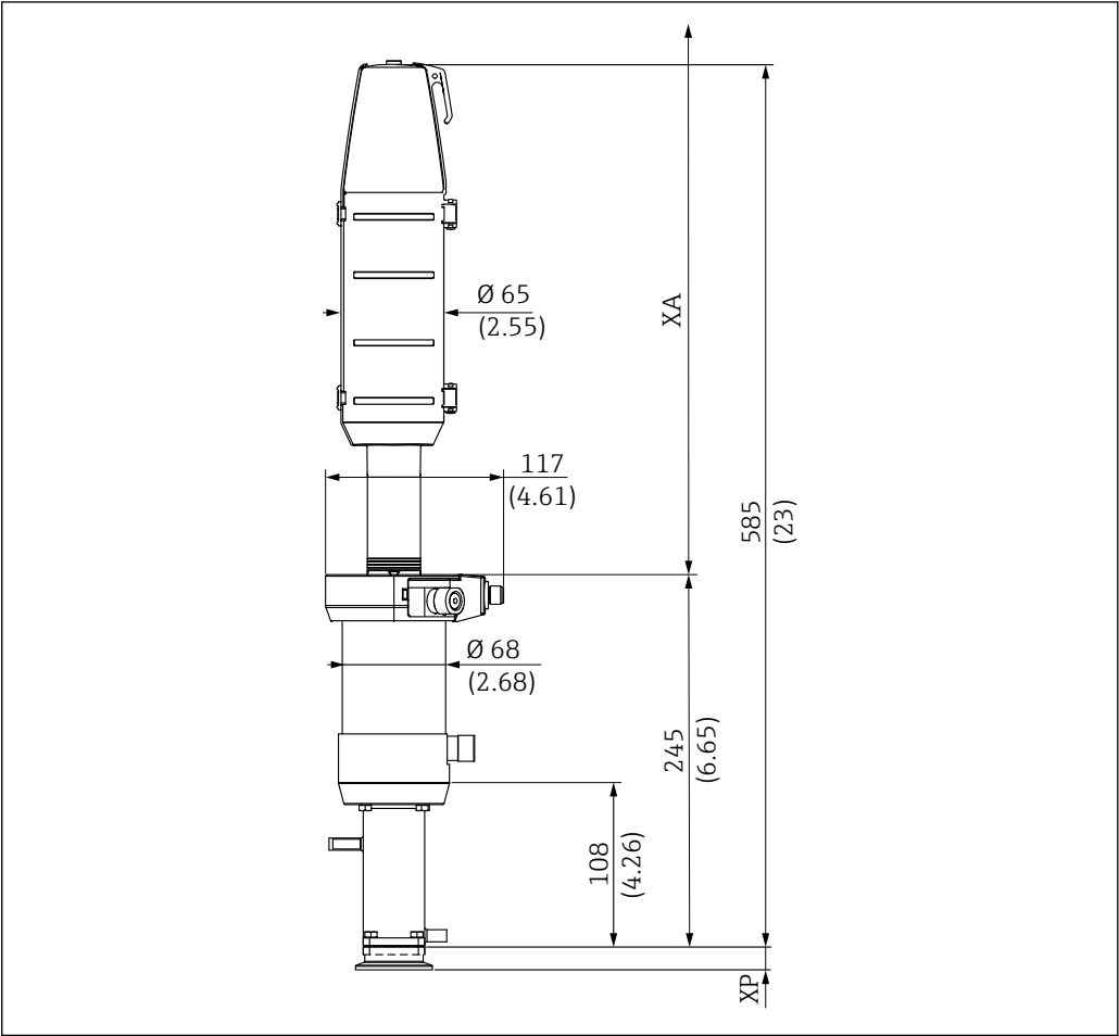
14 Dimensions for long version (78 mm stroke) with pneumatic drive in service position in mm (in) XP Height of particular process connection (see table below) XA Necessary mounting distance for sensor replacement
