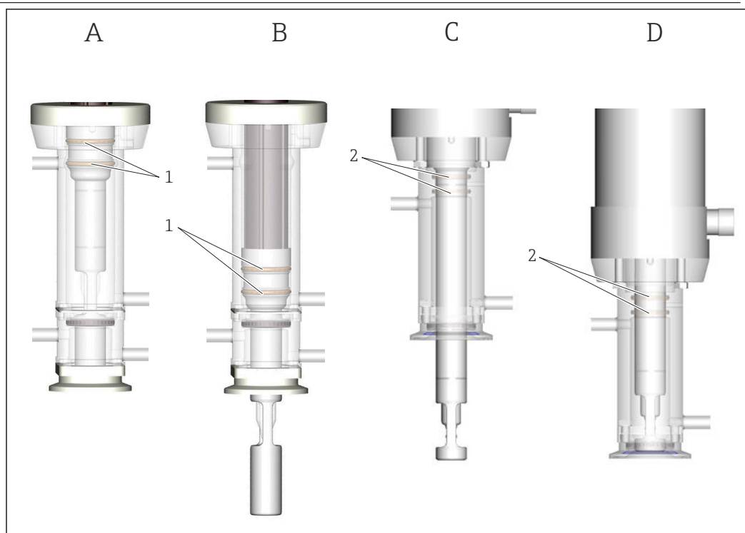
5 Sealing principle
