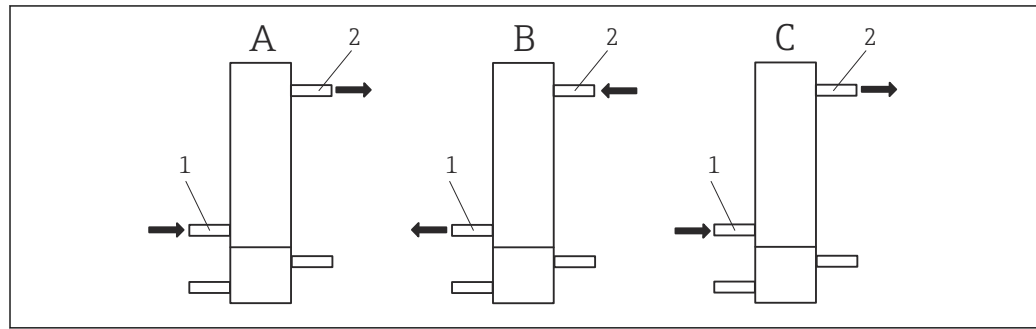
8 Assignment of rinse inlet and outlet
