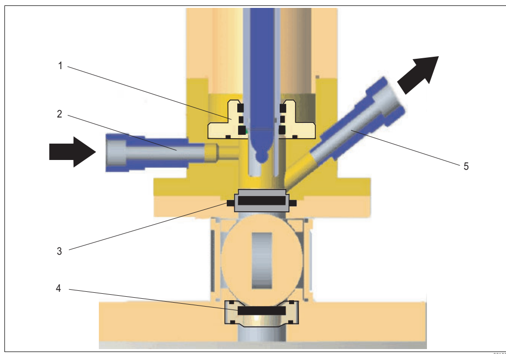
Sealing system
