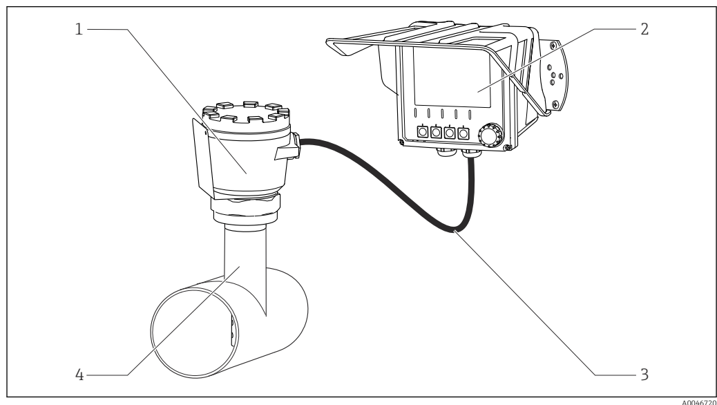
2 Example of a measuring system
