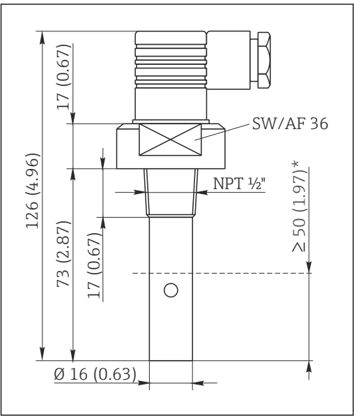
7 Dimensions in mm (in) * Minimum immersion depth
