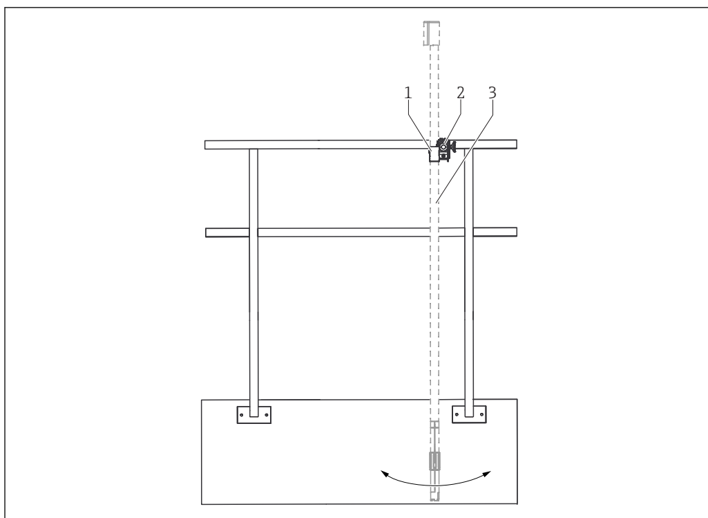
Pendulum holder on rail with immersion pipe
