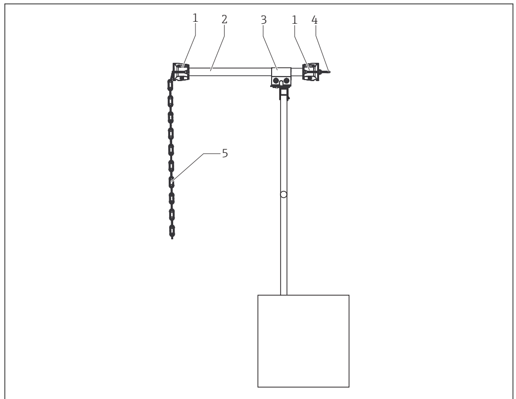
Transverse pipe on rail with chain retainer
