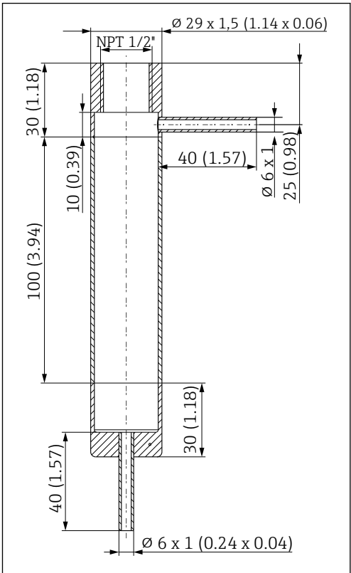
6 Dimensions of CYA21 NPT 1/2". Engineering unit in mm (inch)
