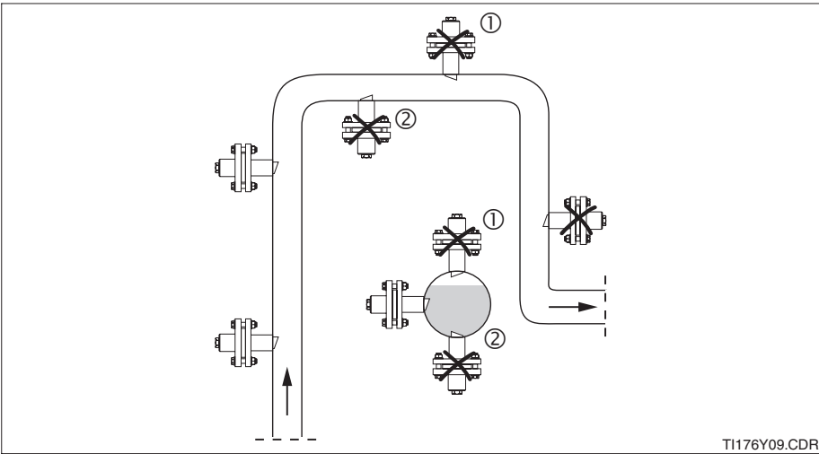
Recommended mounting positions of CUS with CUA 120-A/-B adapter or CUA 461 retractable assembly
