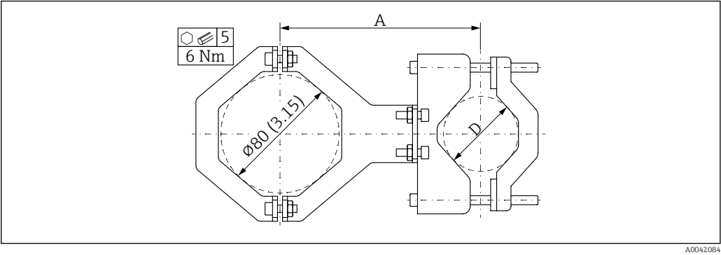
21 Overview of the mounting dimensions
