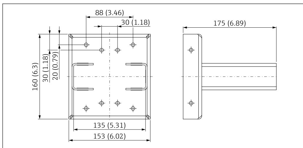
23 Retaining bracket
