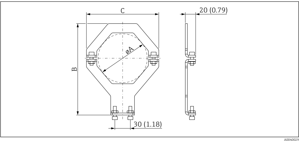
22 Dimensions of mounting clamp (at the device)
