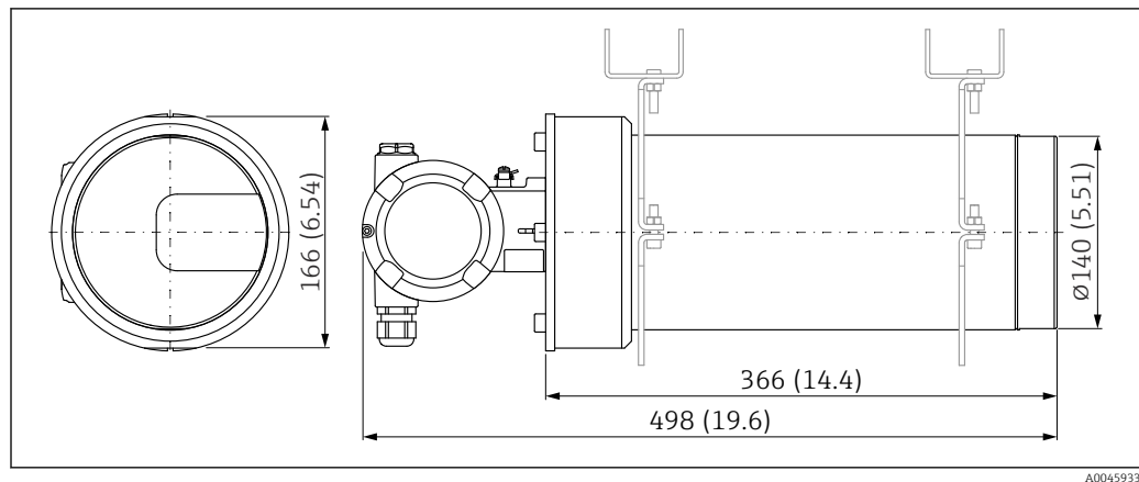
13 Version NaI (TI) 2" with collimator on sensor side
