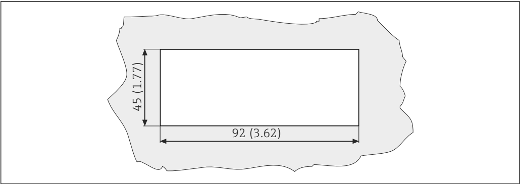
6 Panel cutout. Engineering unit mm (in)
