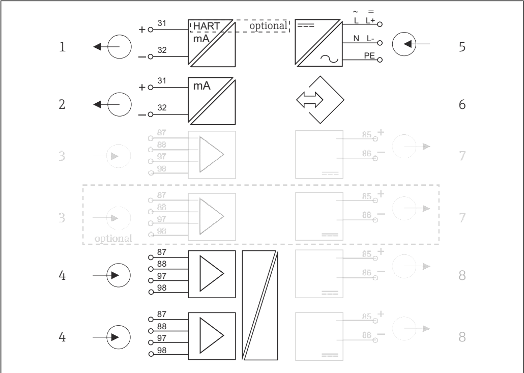
Block circuit diagram CM442 with sensor communication module 2DS Ex-i
