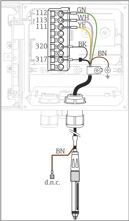
28 In-device view (sensor module)
