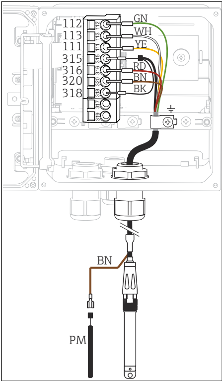
30 In-device view (sensor module)
