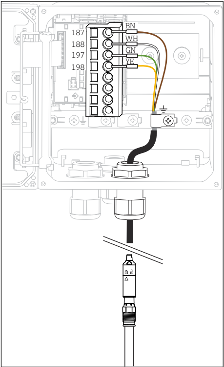
22 In-device view (sensor module)
