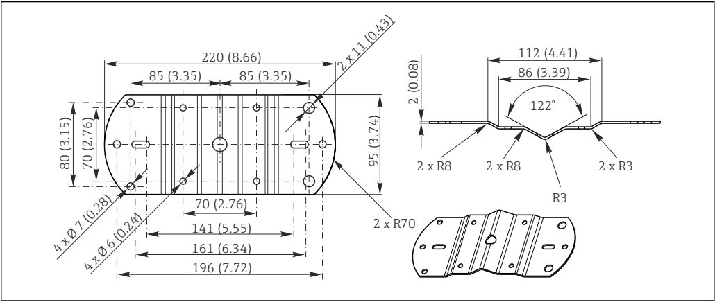
48 Dimensions in mm (inch)
