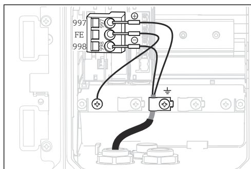
16 In-device view (CPU module)
