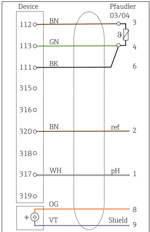
37 Wiring diagram
