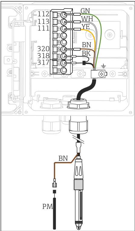
26 In-device view (sensor module)
