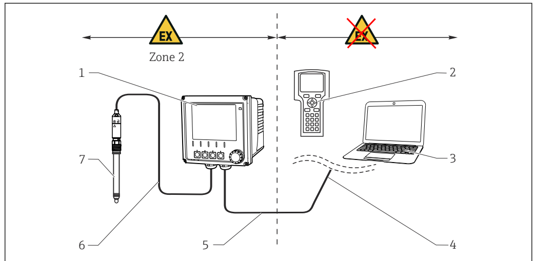
53 Installation in hazardous area Ex nA (ic)
