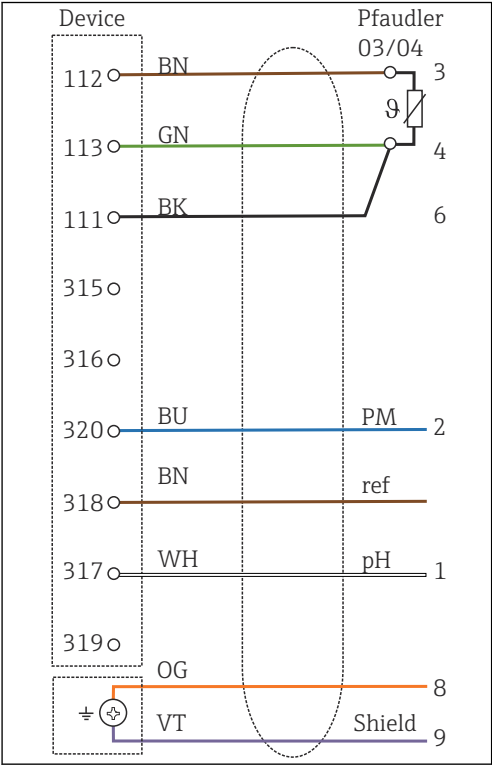
34 Wiring diagram
