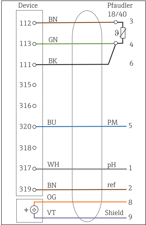
35 Wiring diagram
