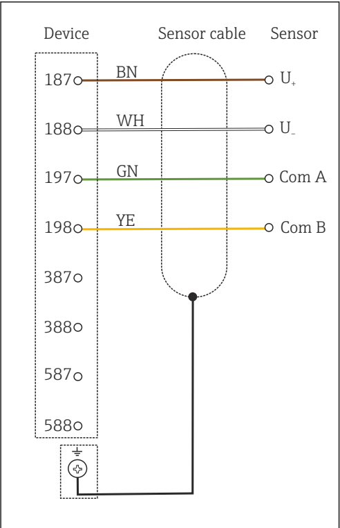
23 Wiring diagram
