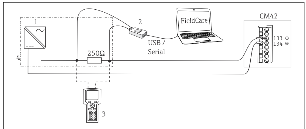
64 HART system integration without PLC
