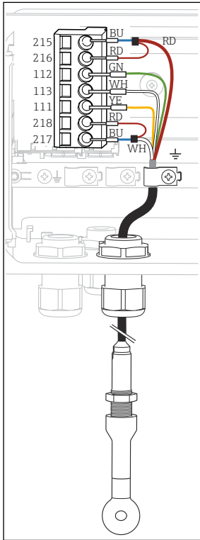
45 In-device view (sensor module)
