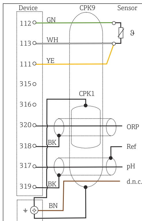
40 Wiring diagram
