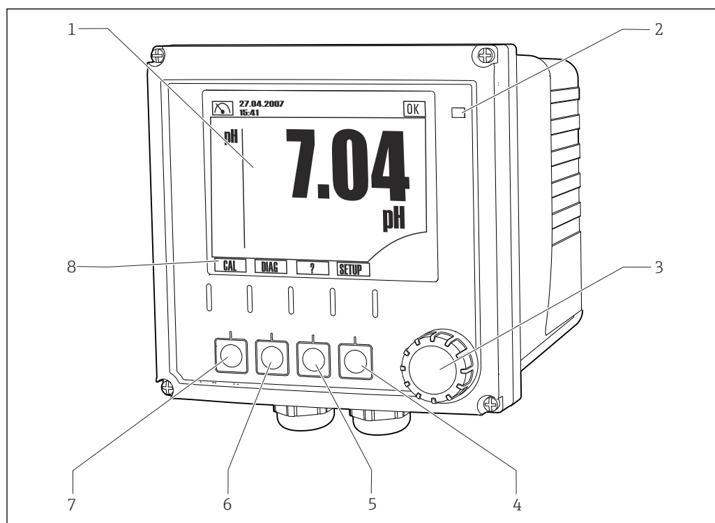
63 Overview of operation
