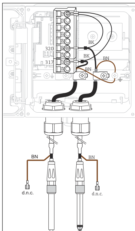
38 In-device view (sensor module)
