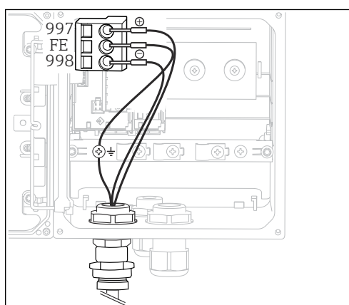
20 In-device view (CPU module)
