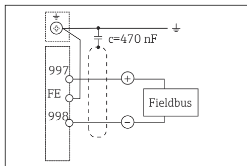
19 Wiring diagram
