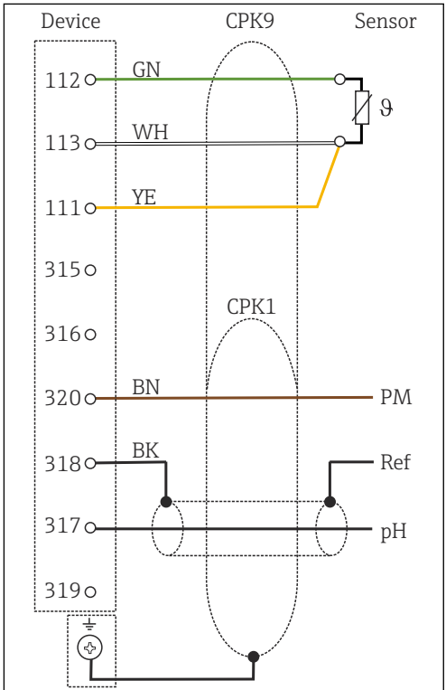
27 Wiring diagram
