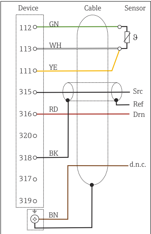
33 Wiring diagram
