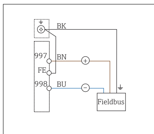
21 Wiring diagram
