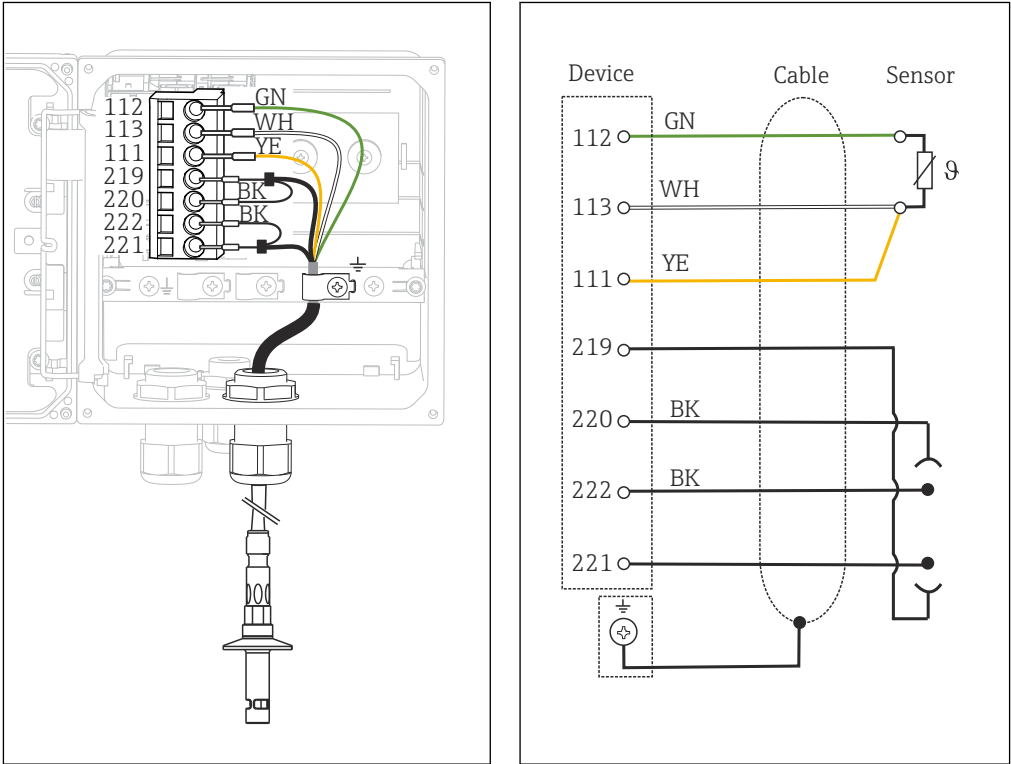
43 In-device view (sensor module)
