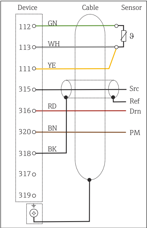
31 Wiring diagram
