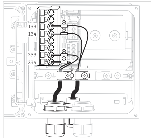
14 In-device view (CPU module)
