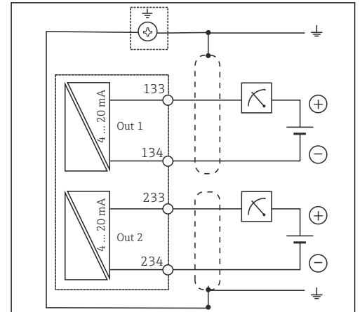
13 Wiring diagram
