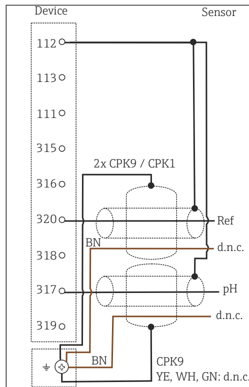
39 Wiring diagram
