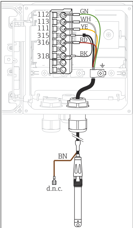
32 In-device view (sensor module)
