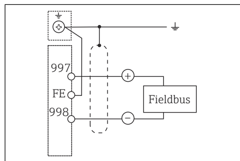
17 Wiring diagram
