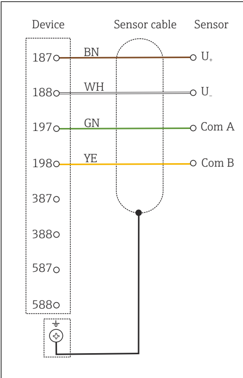
25 Wiring diagram
