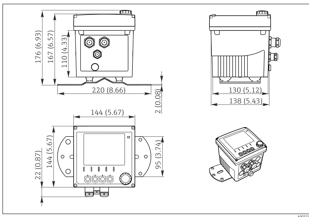
59 Dimensions in mm (inch)
