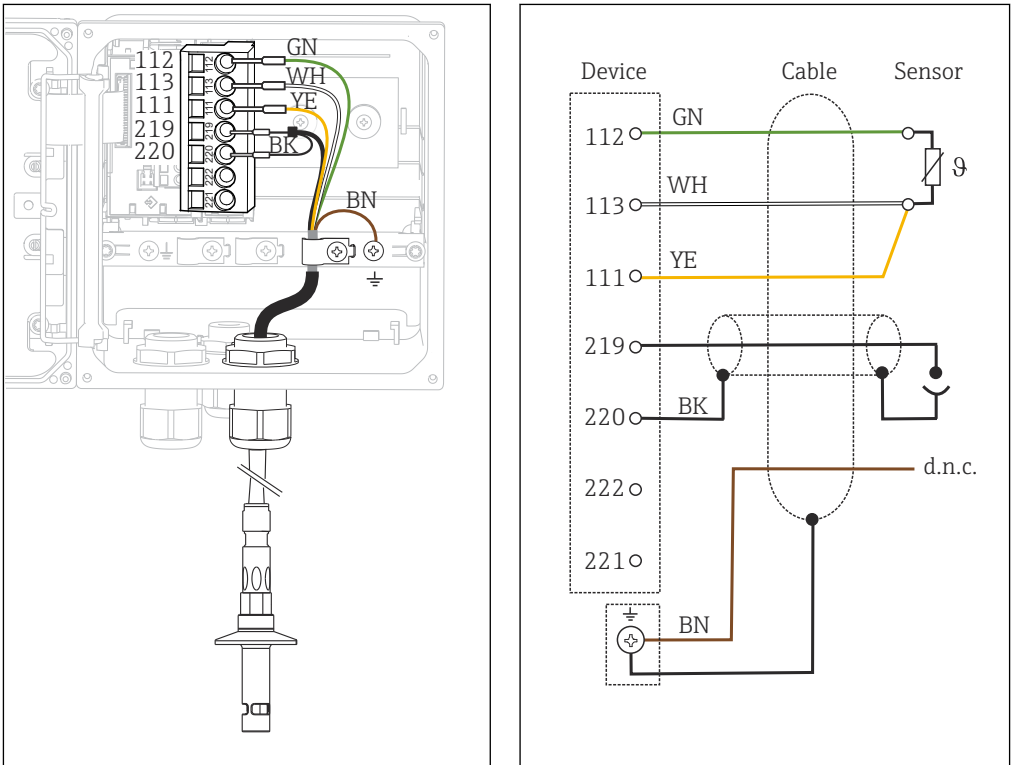
41 In-device view (sensor module)
