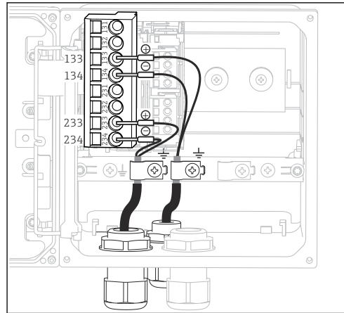
12 In-device view (CPU module)
