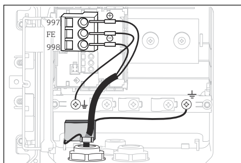
18 In-device view (CPU module)
