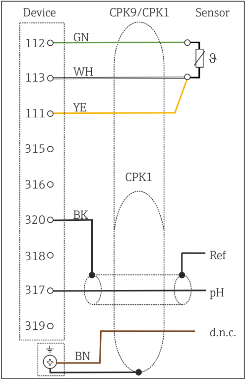
29 Wiring diagram
