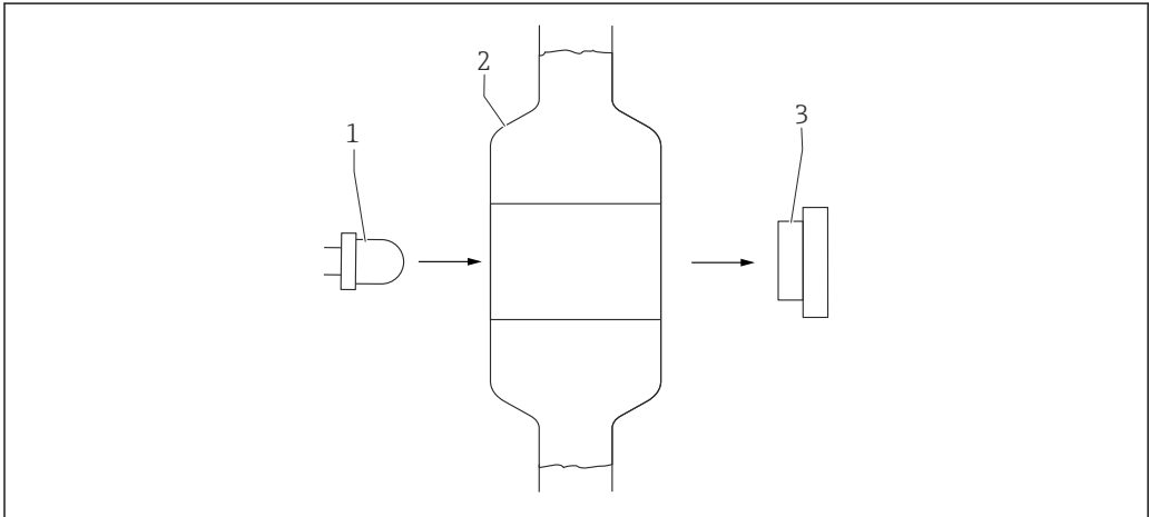
1 Multispectral LED unit (for measurement/reference) 2 Cuvette - mixing and reaction vessel 3 Detector (for measurement/reference)
