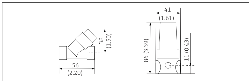
16 1-/2-channel version: filter (left), pressure-reducing valve (right). Unit of measurement mm (in)
