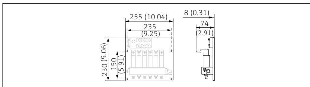
18 4/6-channel version: panel with sample channel switching. Unit of measurement mm (in)
