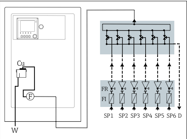
3 4-/6-channel version: Measuring system with upstream pressure relief valves and filters on panel and external sample channel switching on panel
