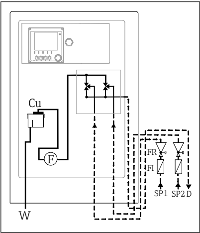
2 1-/2-channel version: Measuring system with upstream pressure relief valves and filters
