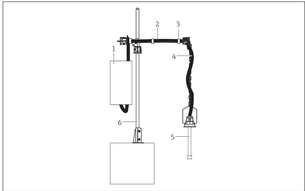
4 Installation with Liquiline System CA80, CAT860 with chain retainer and filter (ceramic)
