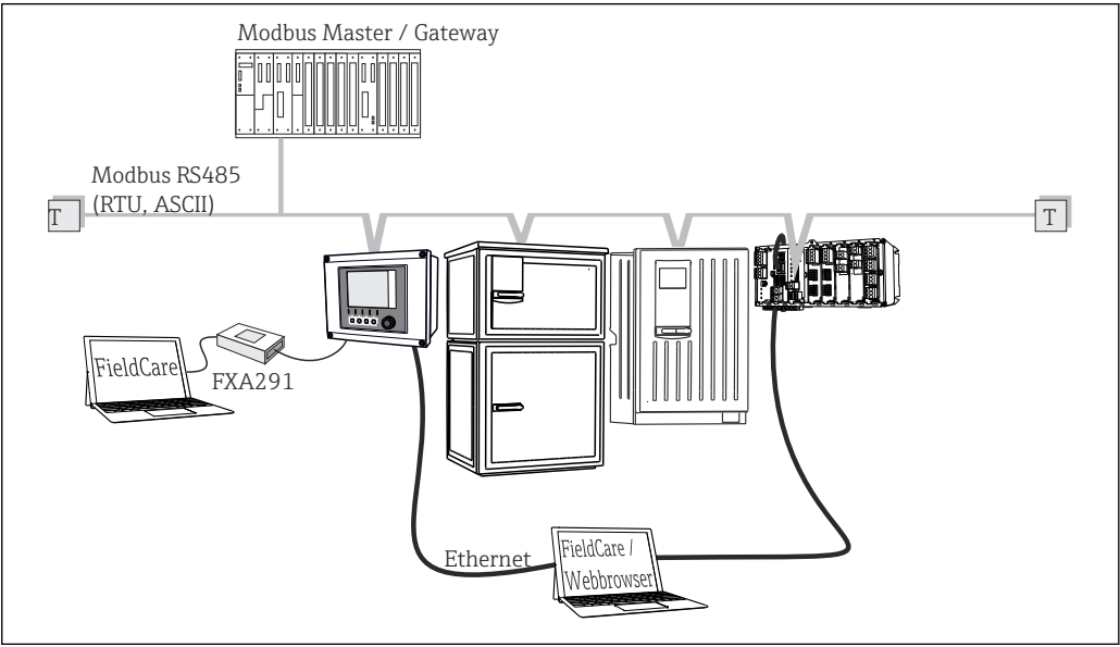
24 Modbus RS485
