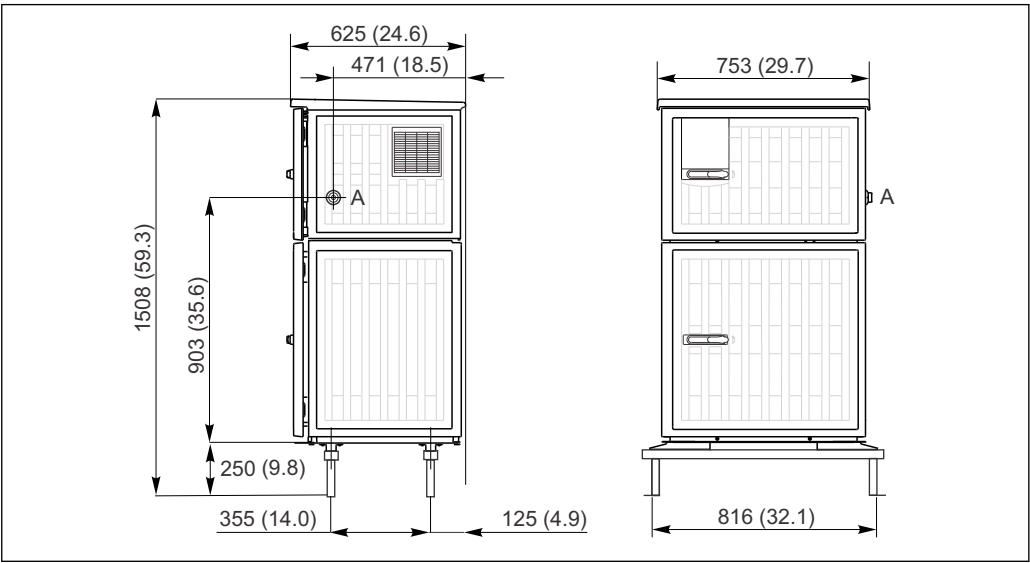
16 Dimensions of Liquistation, plastic version, with stand. Unit of measurement mm (in) A Suction line connection
