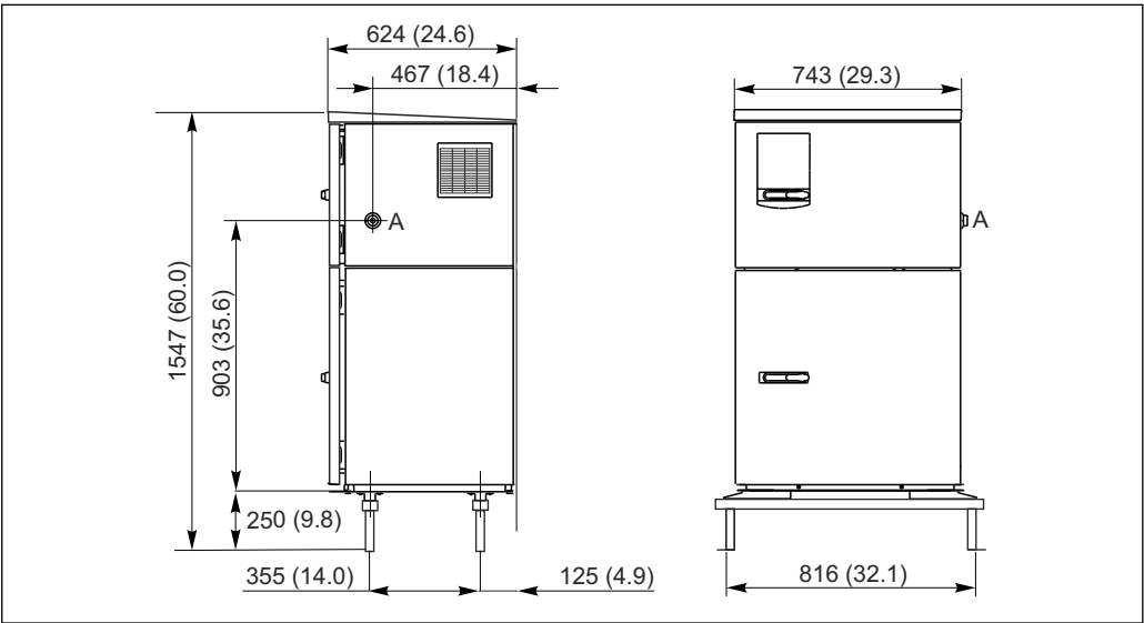
17 Dimensions of Liquistation, stainless steel version, with stand. Unit of measurement mm (in) A Suction line connection
