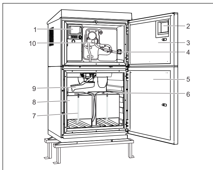
7 Example of a Liquistation, version with peristaltic pump
