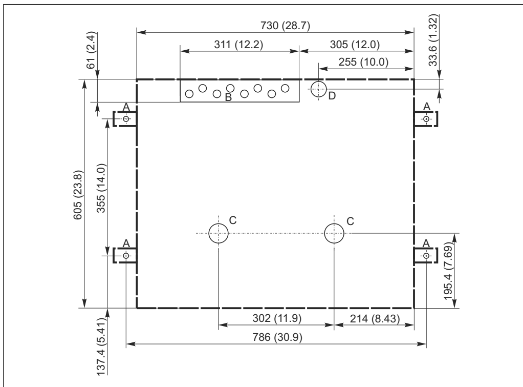
22 Foundation plan. Unit of measurement mm (in)
