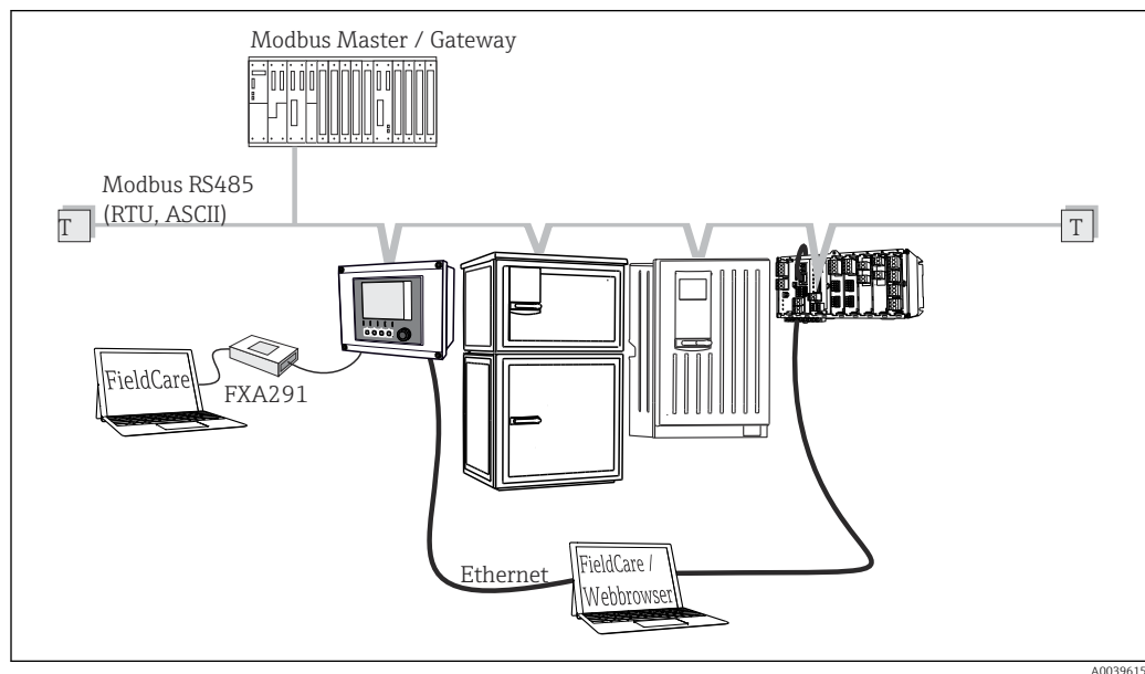
33 Modbus RS485
