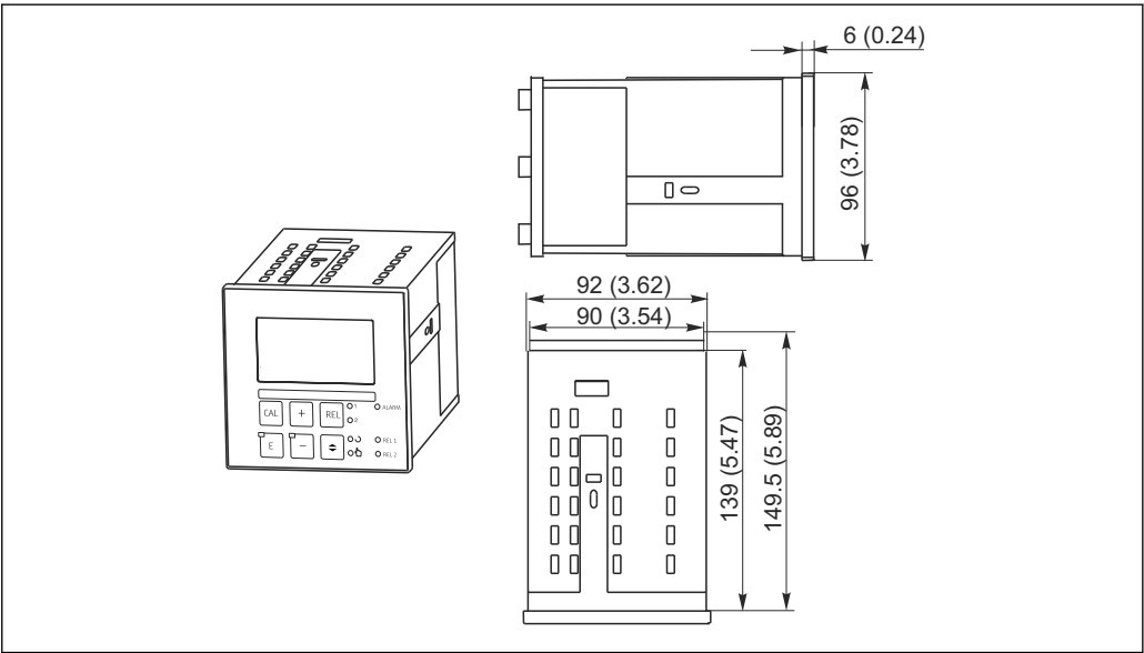
13 Panel-mounted device: dimensions in mm (inch)
