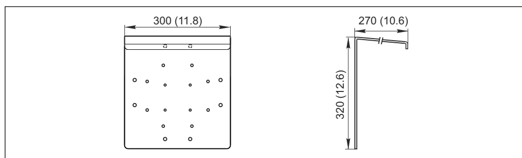
15 Dimensions in mm (inch)
