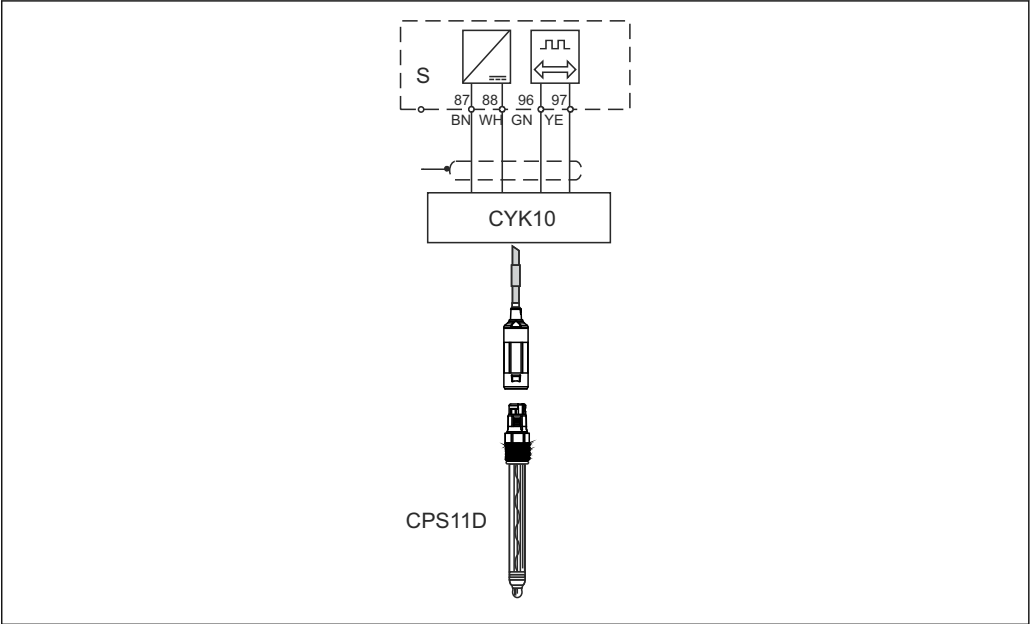
4 Connecting the digital sensor CPS11D with CYK10
