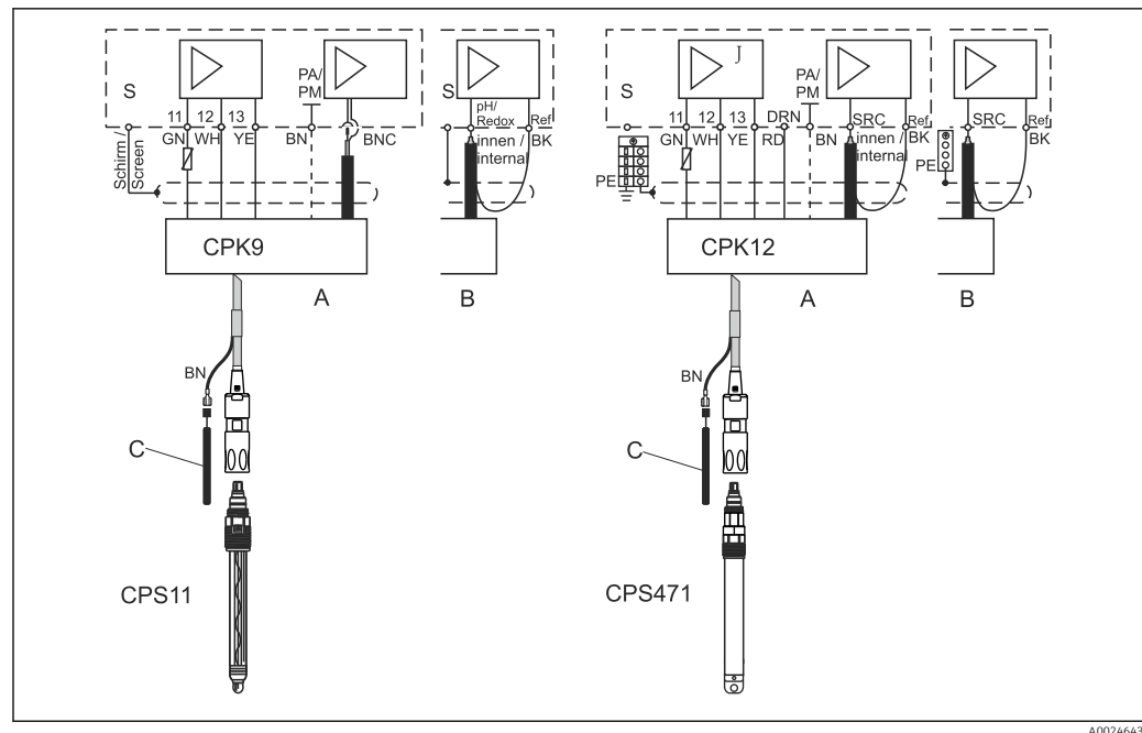
5 Connecting the glass electrode CPS11 with CPK9 (left) and ISFET sensor CPS471 with CPK12 (right)
