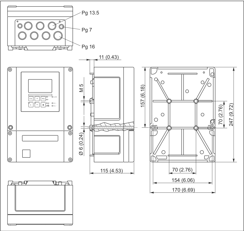
12 Field device: dimensions in mm (inch)
