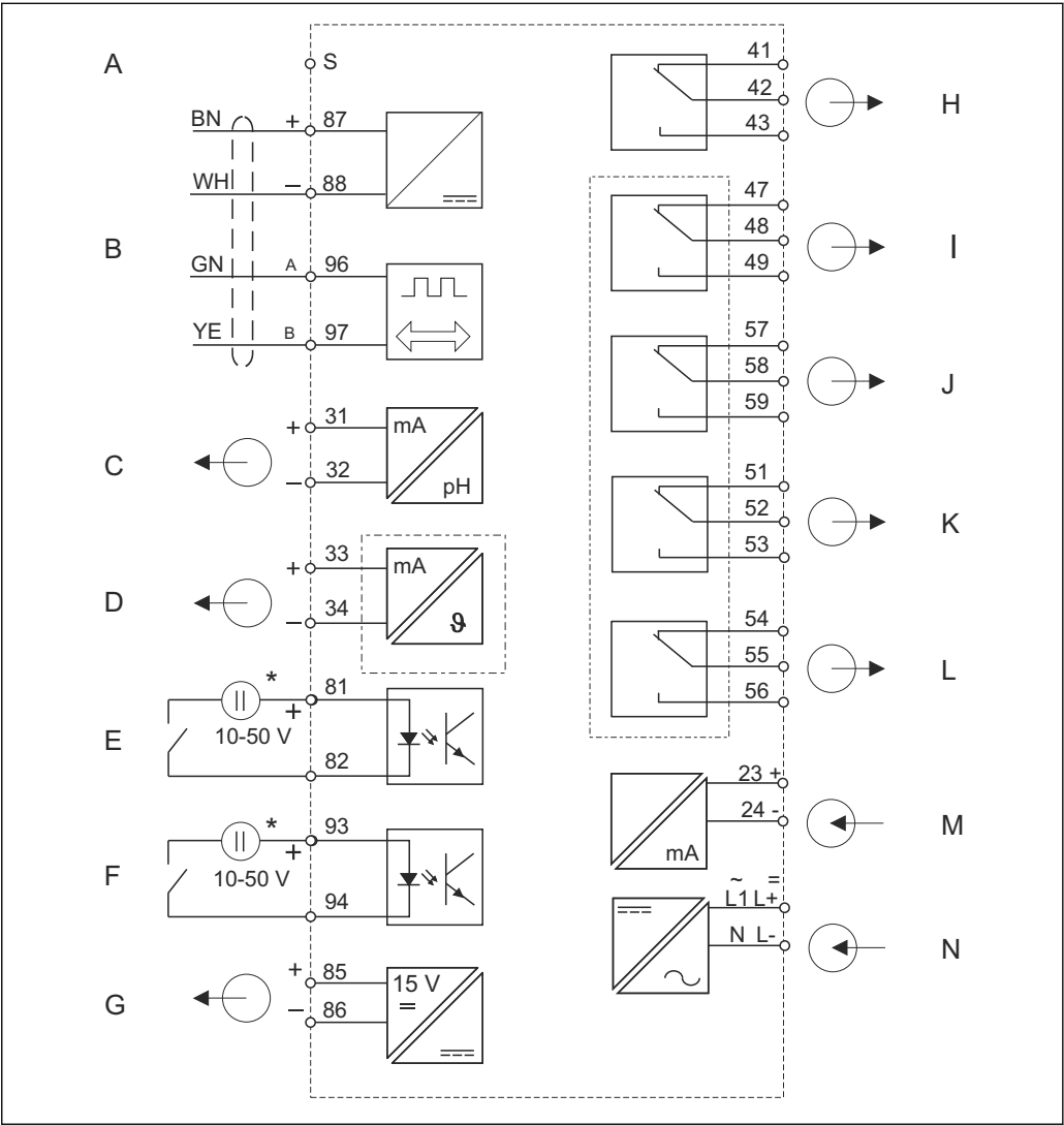
2 Block circuit diagram with Memosens sensors
