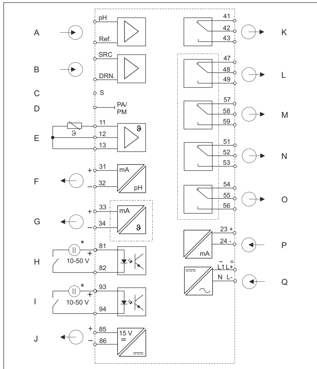
3 Block circuit diagram with analog sensors
