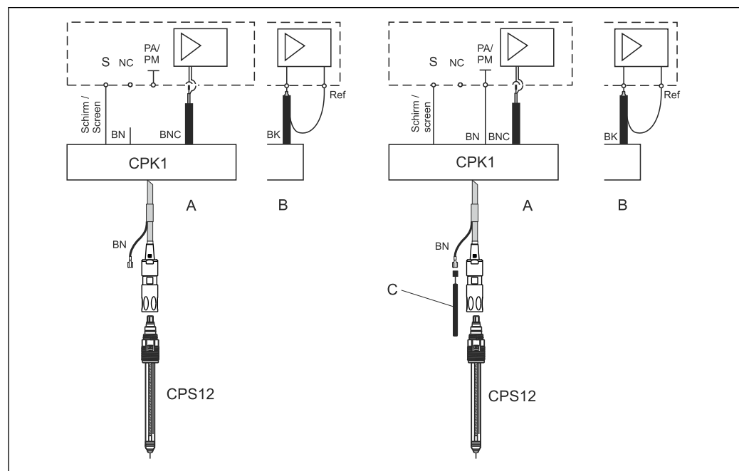
6 Asymmetrical (without PML) and symmetrical (with PML) connection of ORP electrodes
