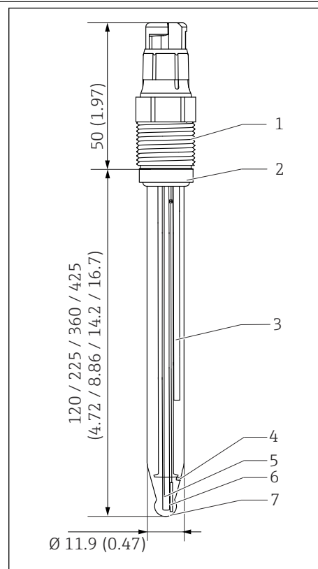
7 CPS61E TU reference system. Engineering unit: mm (in)
