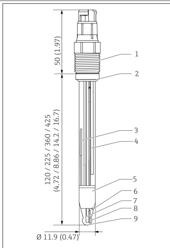
6 CPS61E TP reference system. Engineering unit: mm (in)
