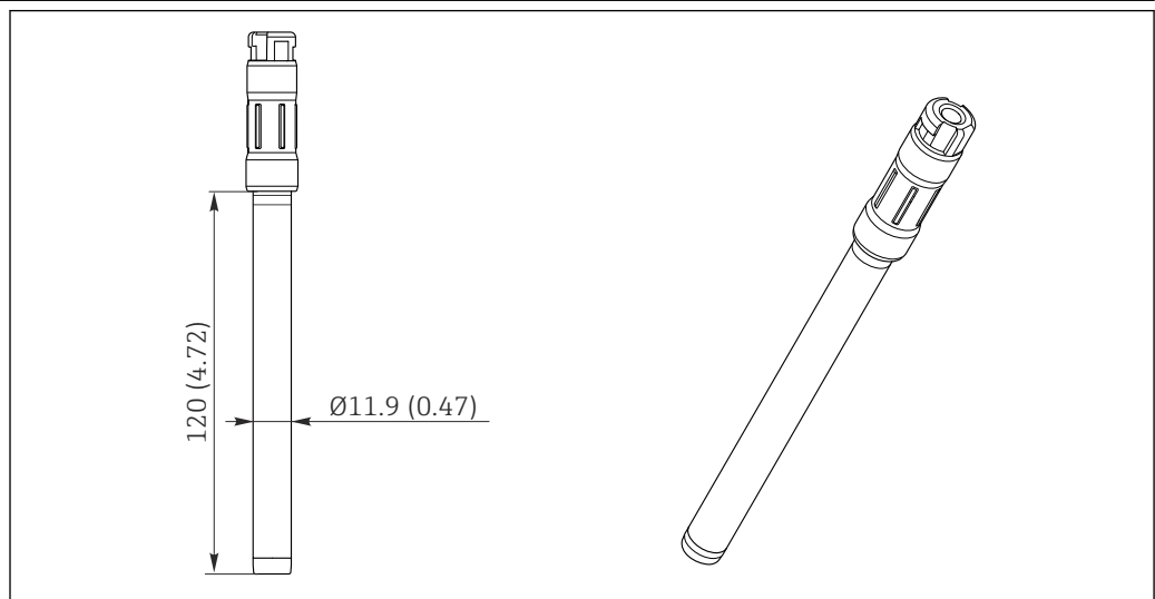
2 Dimensions. Unit of measurement mm (in)
