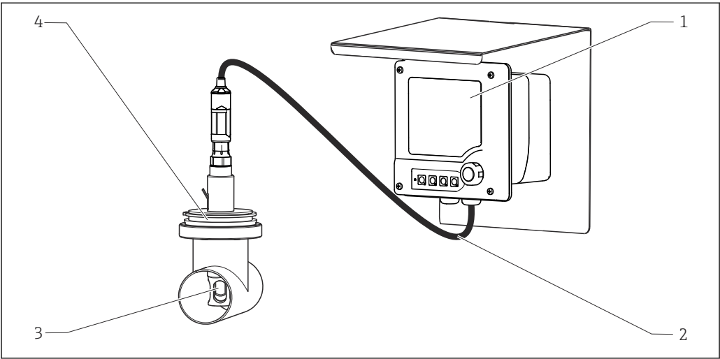
1 Example of a measuring system with Memosens COS22E 1 Liquiline CM42 2 Measuring cable CYK10 3 Oxygen sensor Memosens COS22E 4 Permanent installation assembly CPA842
