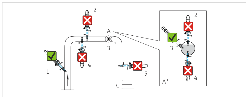
5 Suitable and unsuitable installation positions for Memosens COS22E
