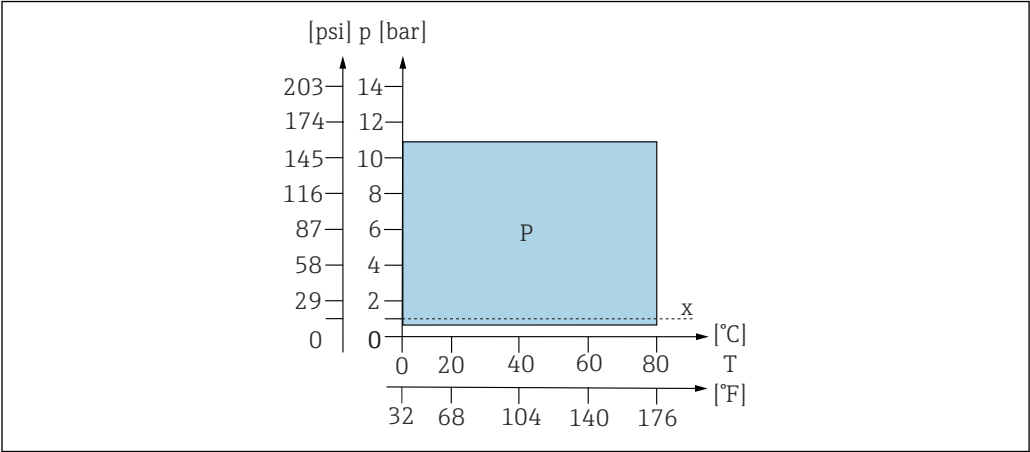
5 Pressure/temperature ratings
