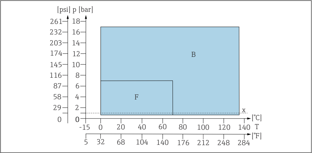
5 Pressure/temperature ratings
