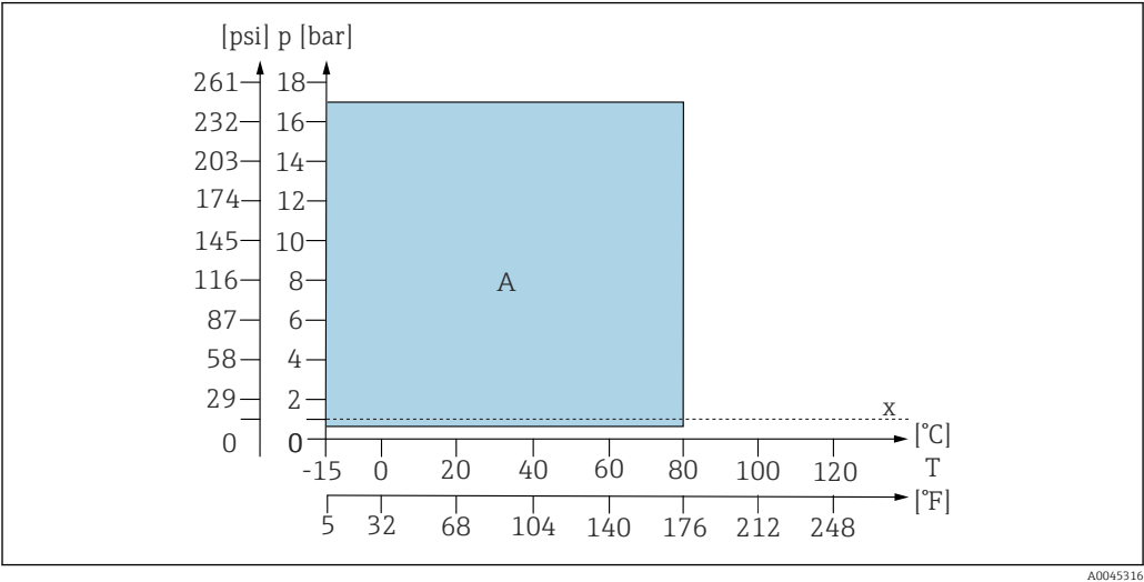
4 Pressure/temperature ratings
