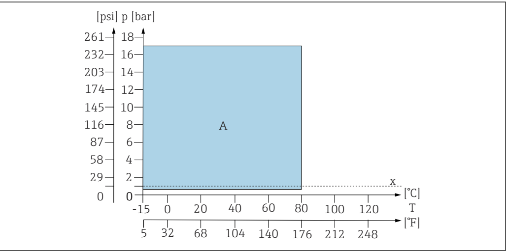
4 Pressure/temperature ratings
