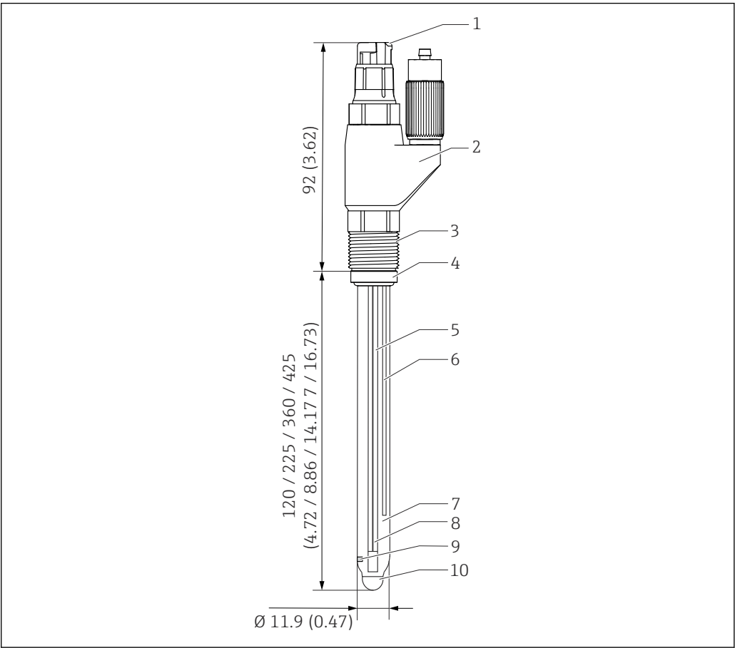
7 CPS42E with hose connection. Engineering unit: mm (in)
