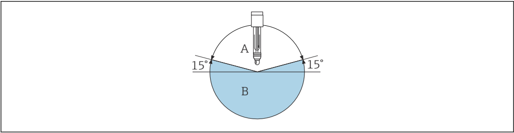
3 Installation angle at least 15° from the horizontal A Permitted orientation B Forbidden orientation
