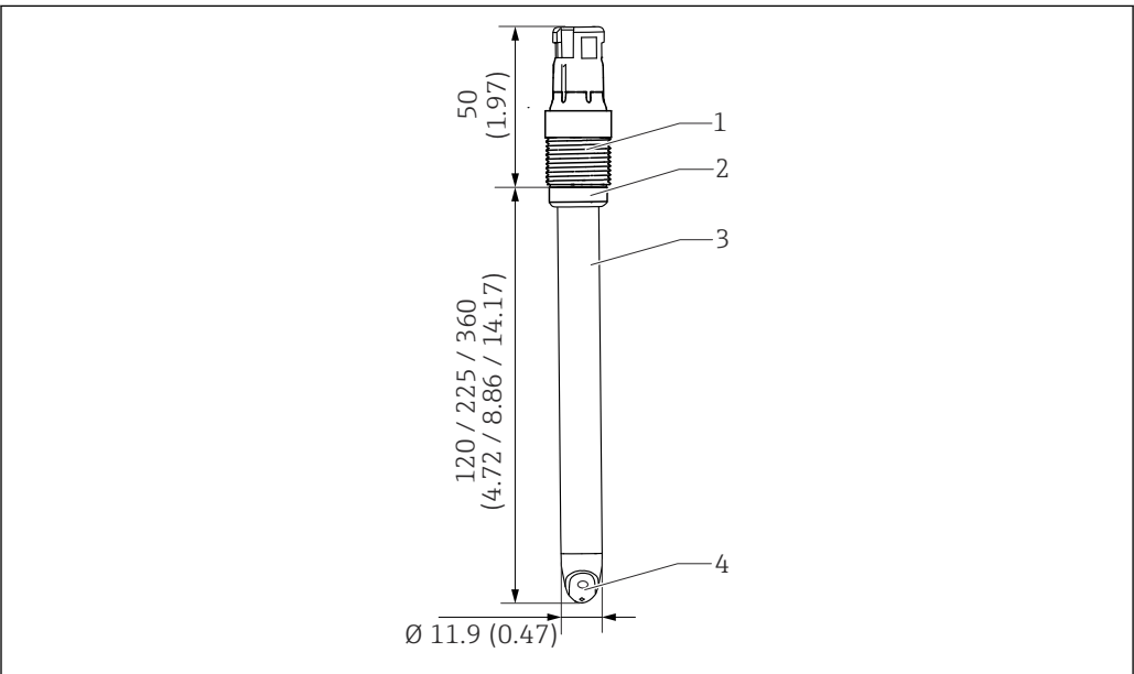
11 Sensor with Memosens plug-in head. Engineering unit: mm (in)
