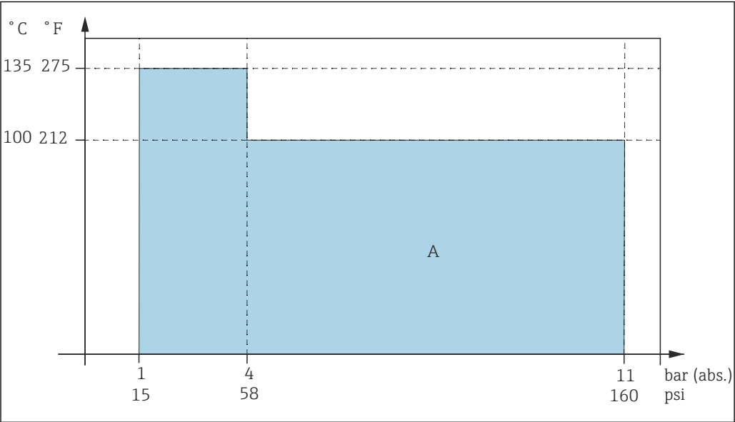
10 Pressure/temperature rating
