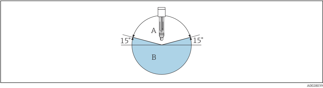
3 Installation angle at least 15° from the horizontal
