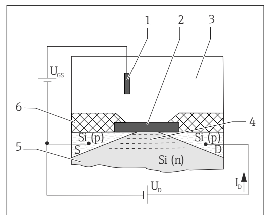
2 ISFET principle
