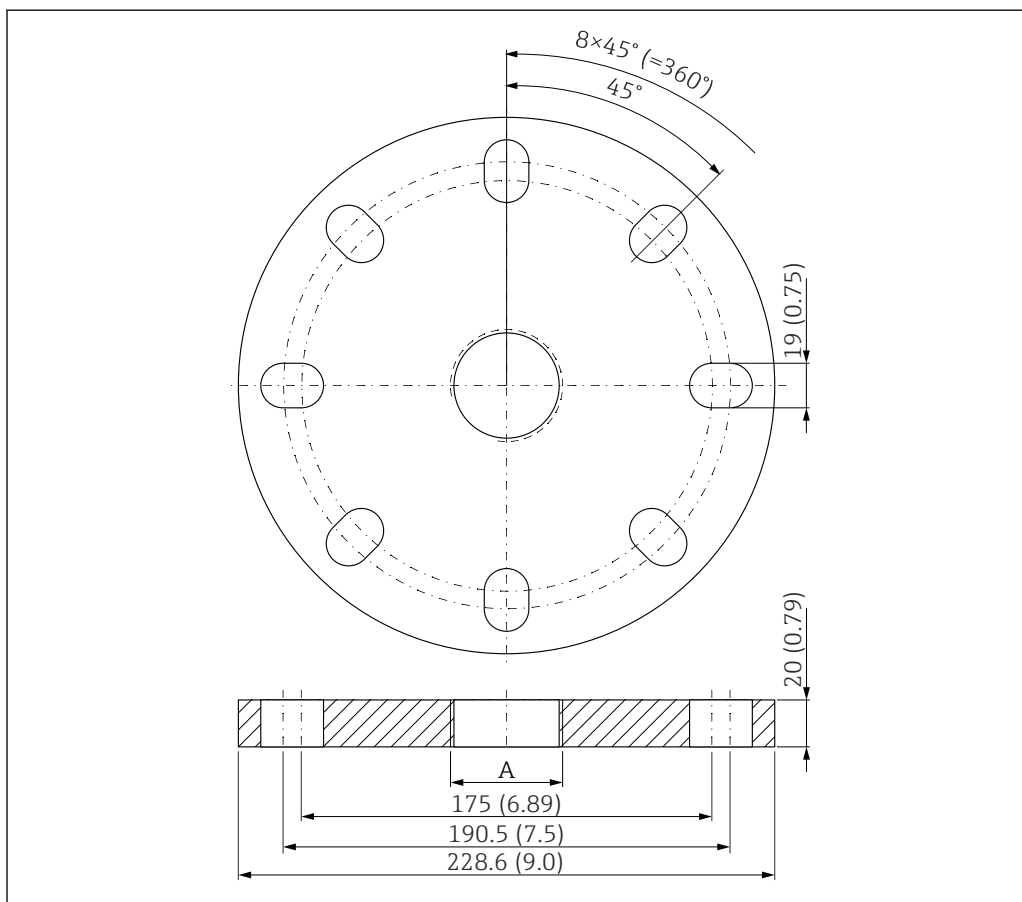
39 Dimensions of UNI flange 4"/DN100/100, engineering unit: mm (in)
