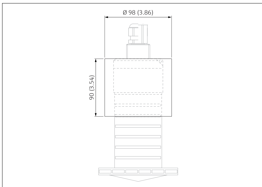
35 Dimensions of weather protection cover, engineering unit: mm (in)
