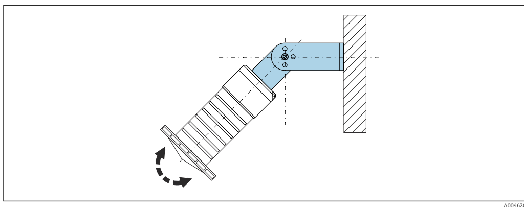
19 Installation with mounting bracket, adjustable
