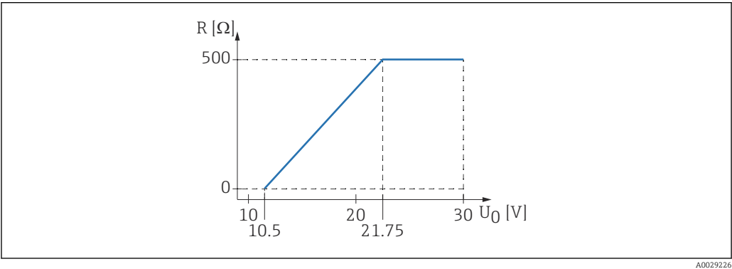
3 Maximum load R , depending on supply voltage U_0 of power supply unit
