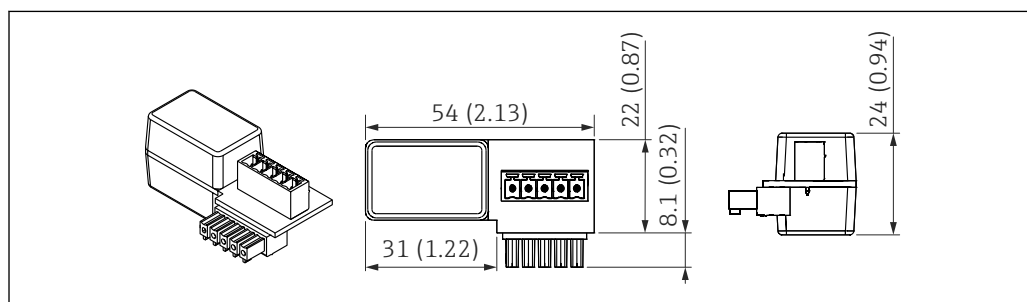
52 Dimensions of HART communication resistor, engineering unit: mm (in)
