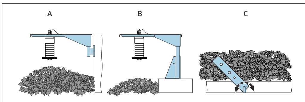
20 Cantilever installation, with pivot
