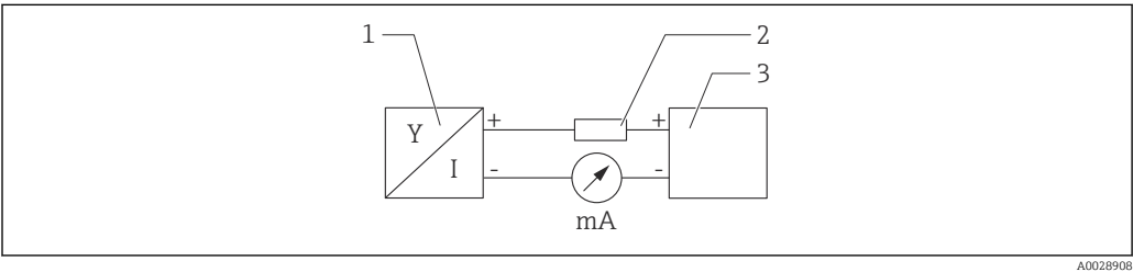
4 Block diagram of HART connection
