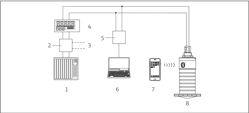
34 Options for remote operation via HART protocol
