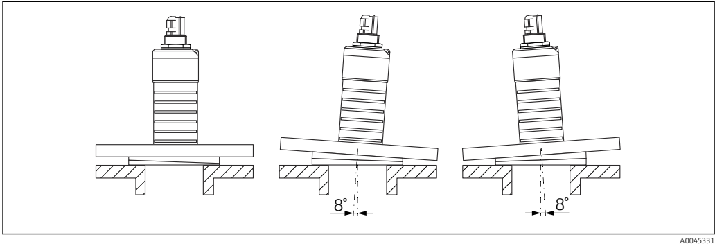
24 Micropilot FMR20 with adjustable flange seal
