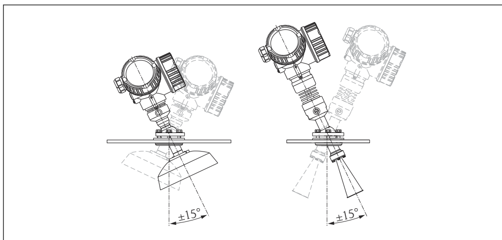
24 Micropilot FMR57 with alignment unit
