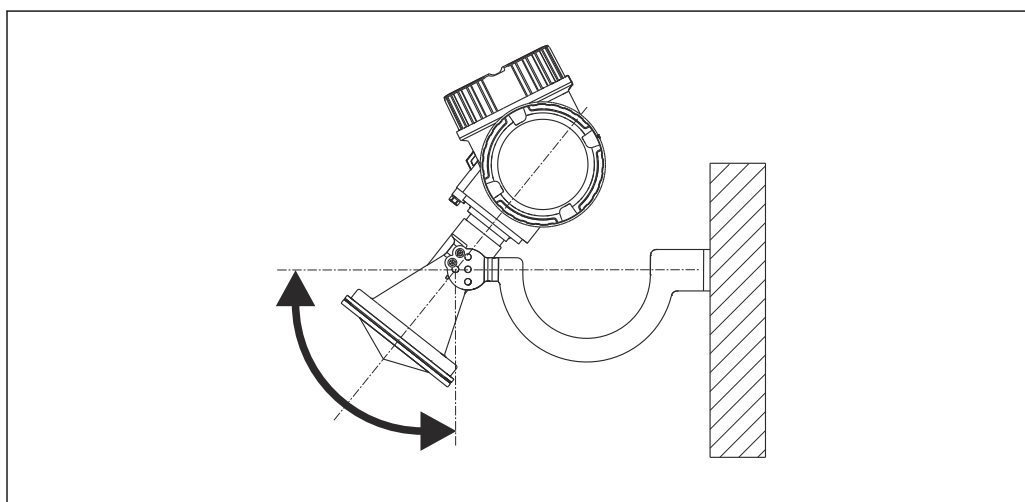
21 Mounting the horn antenna with a mounting bracket
