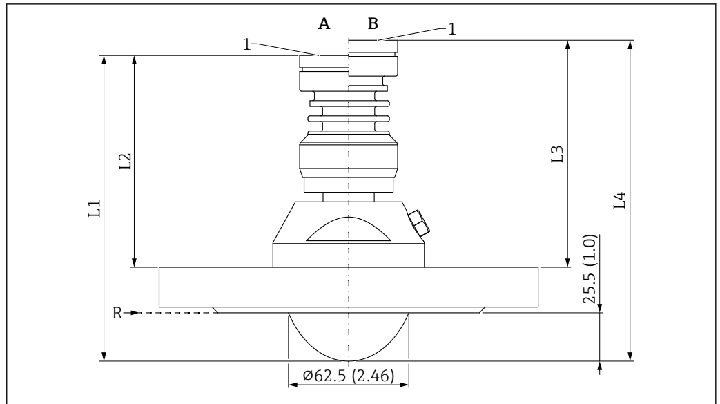
51 Dimensions of antenna flush mount, PTFE, 80 mm (3 in), with standard flange and purge air connection . Unit of measurement mm (in)
