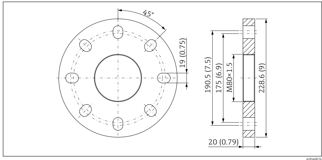
49 UNI flange 4"/DN100/100A for Drip-off antenna, PTFE, 50 mm (2 in) with purge air connection. Unit of measurement mm (in)
